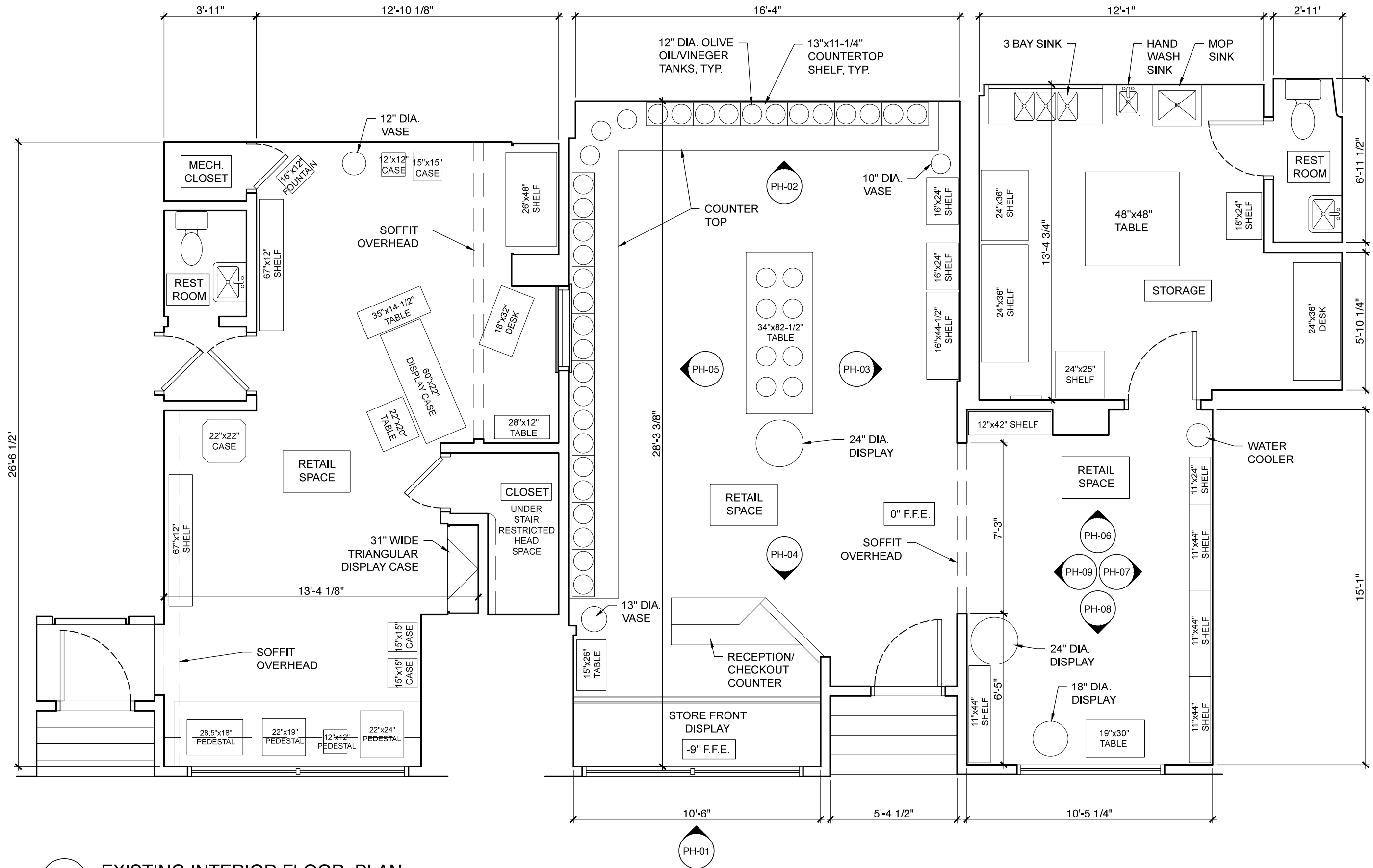
1 EXISTING INTERIOR FLOOR PLAN 1/4" = 1'-0"
