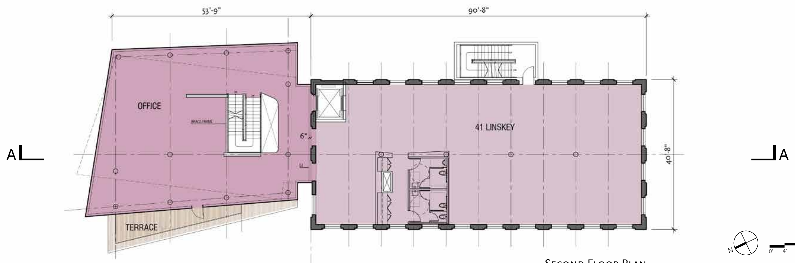
SECOND & THIRD FLOOR PLAN
