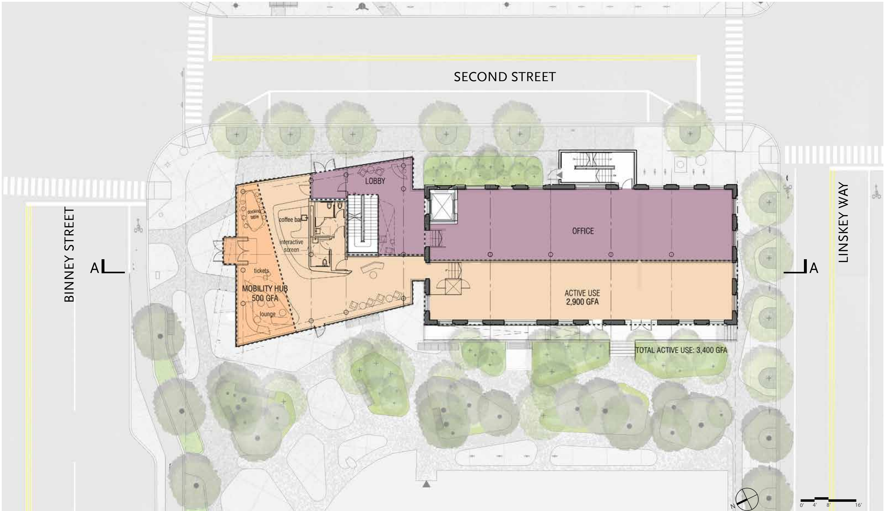
GROUND FLOOR PLAN_OPTION 2
